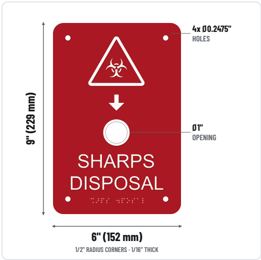
LAYOUT & DIMENSIONS
